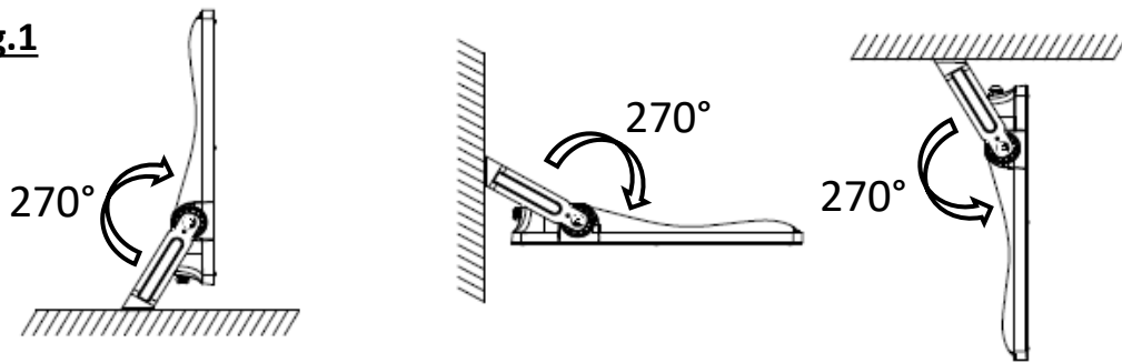
Horizontal Installation
